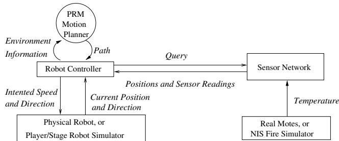
Fig. 1. System overview.
