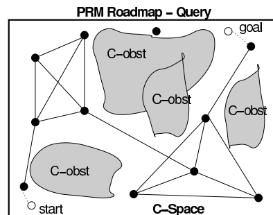
Fig. 3. Querying a PRM roadmap (C-space).
