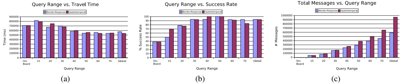
Fig. 5. Experimental results for simulated sensor network using different query strategies. (a) Travel time of the robot. (b) Success rate of the robot reaching the goal. (c) Number of messages sent.
